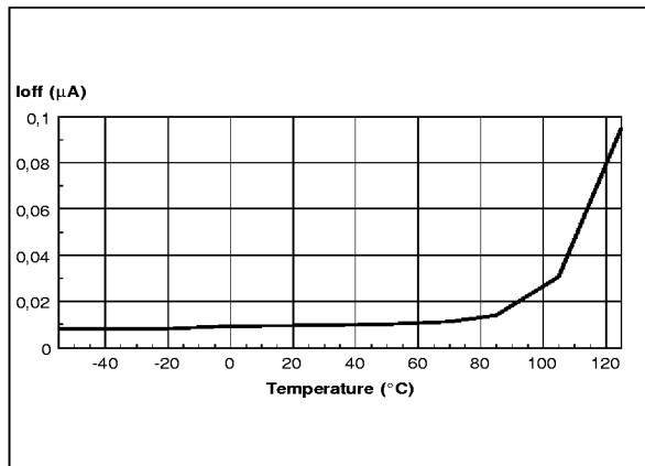
OFF-STATE CATHODE CURRENT vs TEMPERATURE
