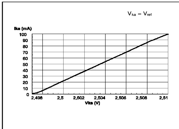
CATHODE CURRENT vs CATHODE VOLTAGE (detailed version)
