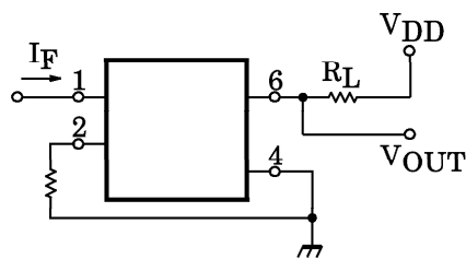
(Note 3) : SWITCHING TIME TEST CIRCUIT
