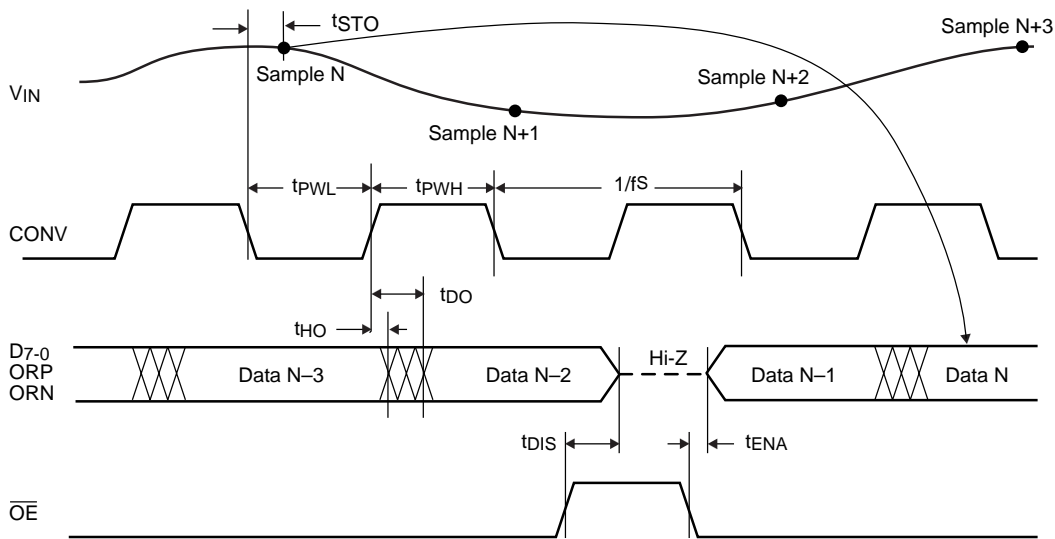
Figure 2. Conversion Timing
