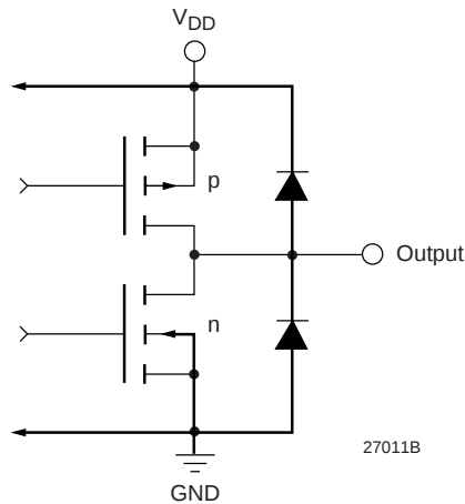
Figure 12. Equivalent Output Circuit
