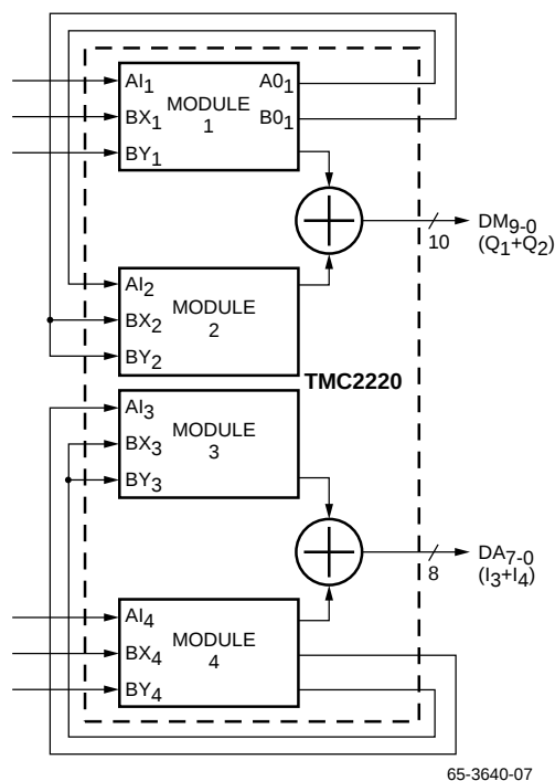
Figure 4. Dual 64 x 1 Configuration
