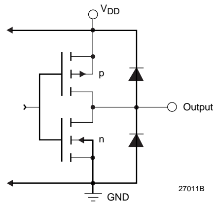
Figure 3. Equivalent Digital Output Circuit
