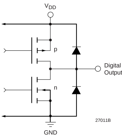
Figure 38. Equivalent Digital Output
