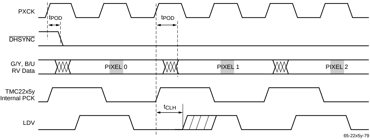
Figure 42. Output Timing Parameters
