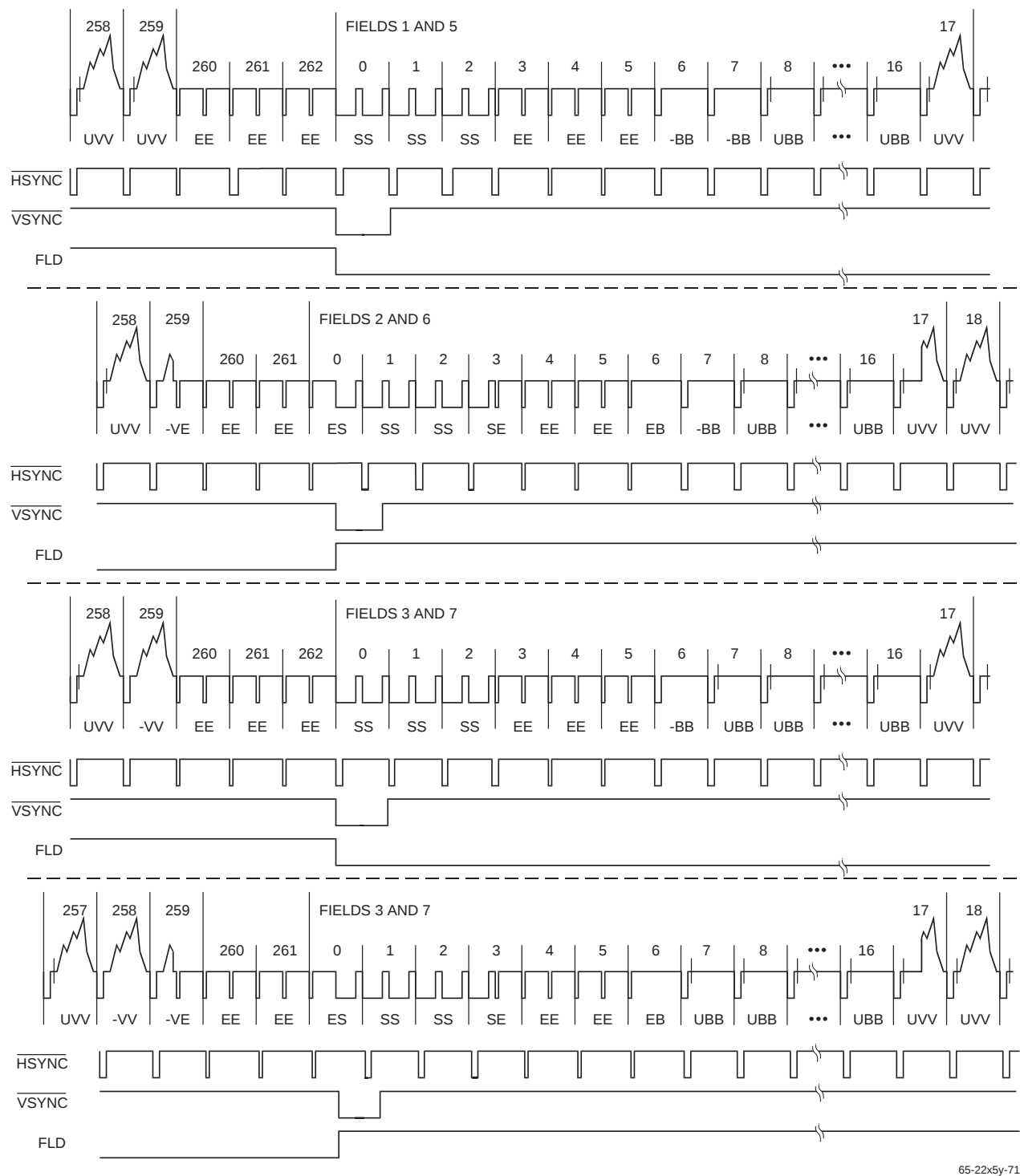
Figure 30. PAL-M Vertical Interval
