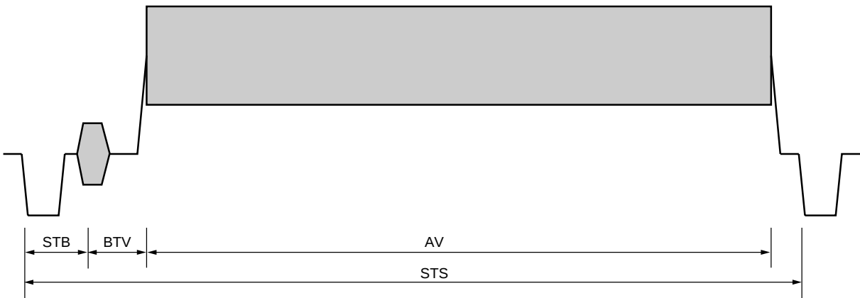
Figure 27. Horizontal Timing
