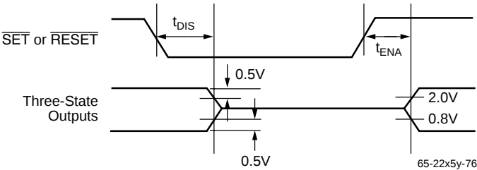
Figure 39. Threshold Levels for Three-state
