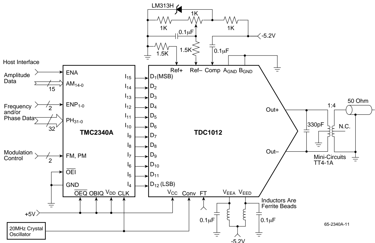
Figure 5. Frequency Synthesizer
