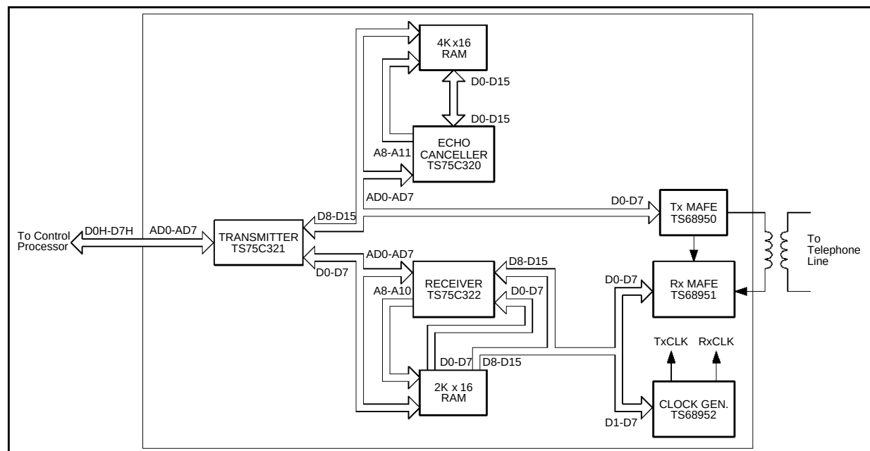
Figure 5 : Hardware Architecture
