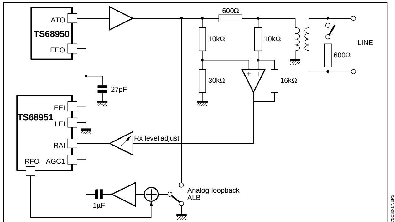
Figure 9 : Analog Path
