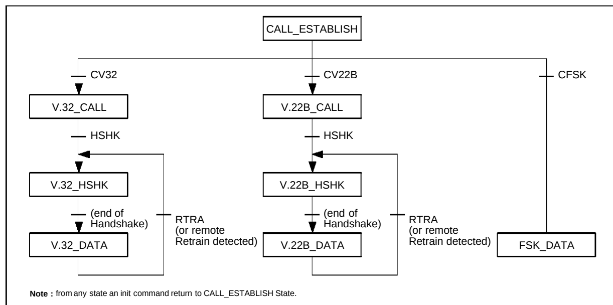
Figure 9 : State Diagram
