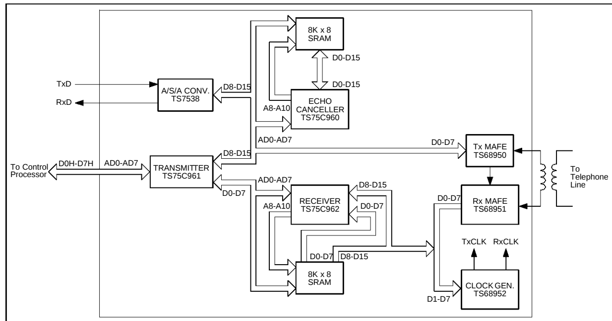
Figure 5 : Hardware Architecture
