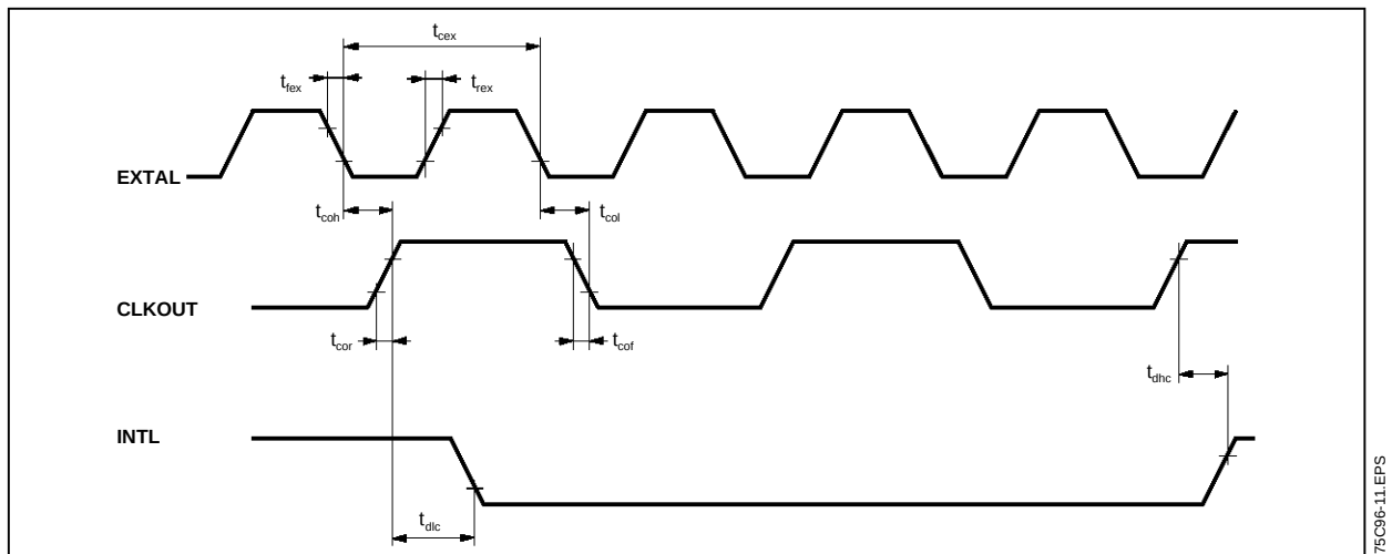
Figure 2 : Clock Timing
