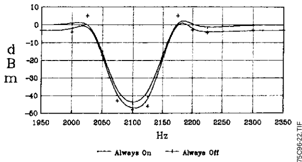
Figure 12 : 2100 Answer Tone Detector
