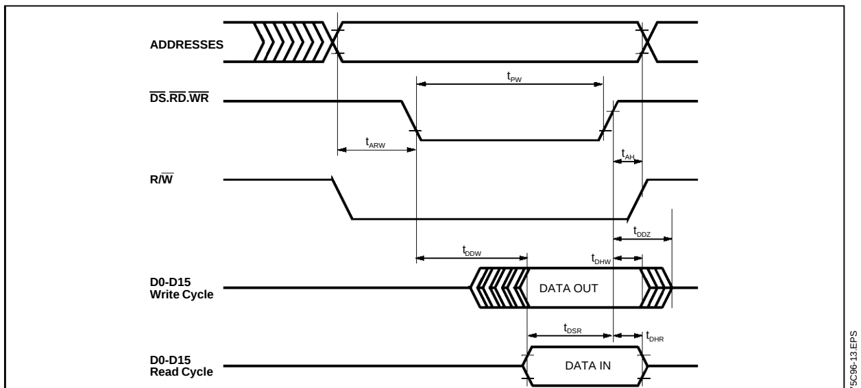
Figure 3 : Local Bus Timing Diagram
