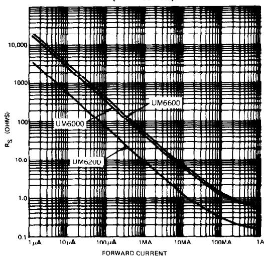
TYPICAL SERIES RESISTANCE VS FORWARD CURRENT ( F = 100\text{MHz} )
