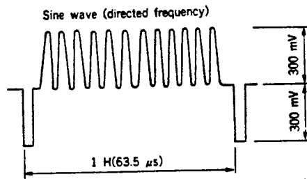
Fig. 1 TEST SIGNAL OF FR PCA , APSP, FRY(SHP)1, FRY(SHP)2, AND V NSHP
