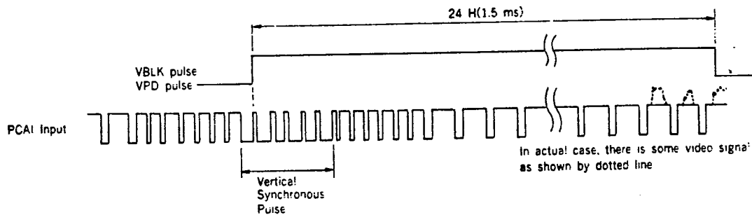
Fig. 3 SIGNAL TIMING OF PW VBLK , AND PW VPD
