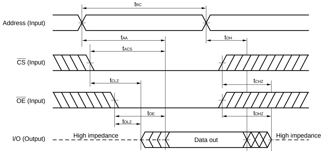
Read Cycle Timing Chart
