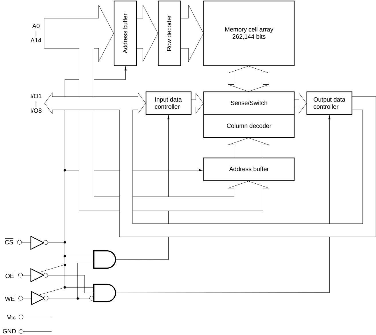
Block Diagram
