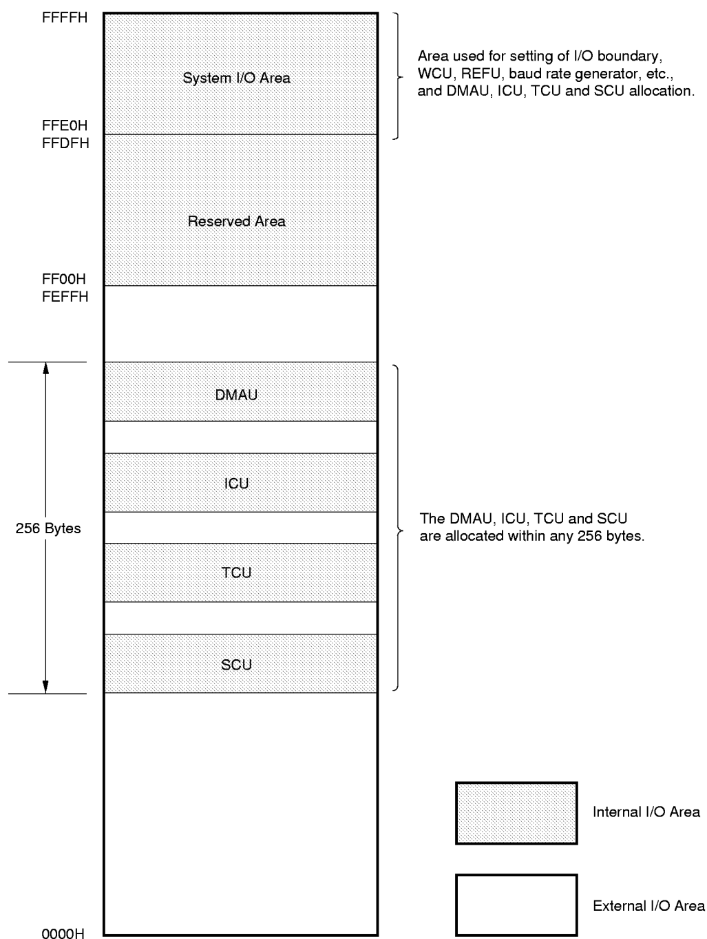
Figure 2-3. I/O Map
