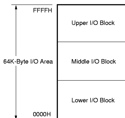
Figure 7-2. Example of I/O Space Division
