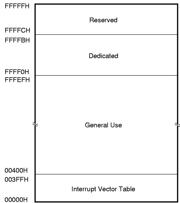
Figure 2-2. Interface with Memory (1/2)
