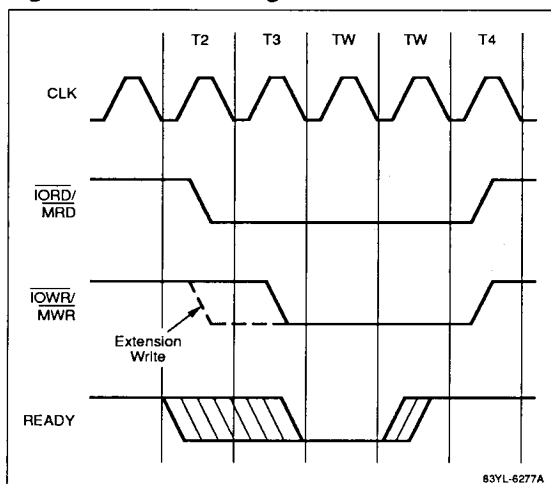
Figure 9. READY Timing
