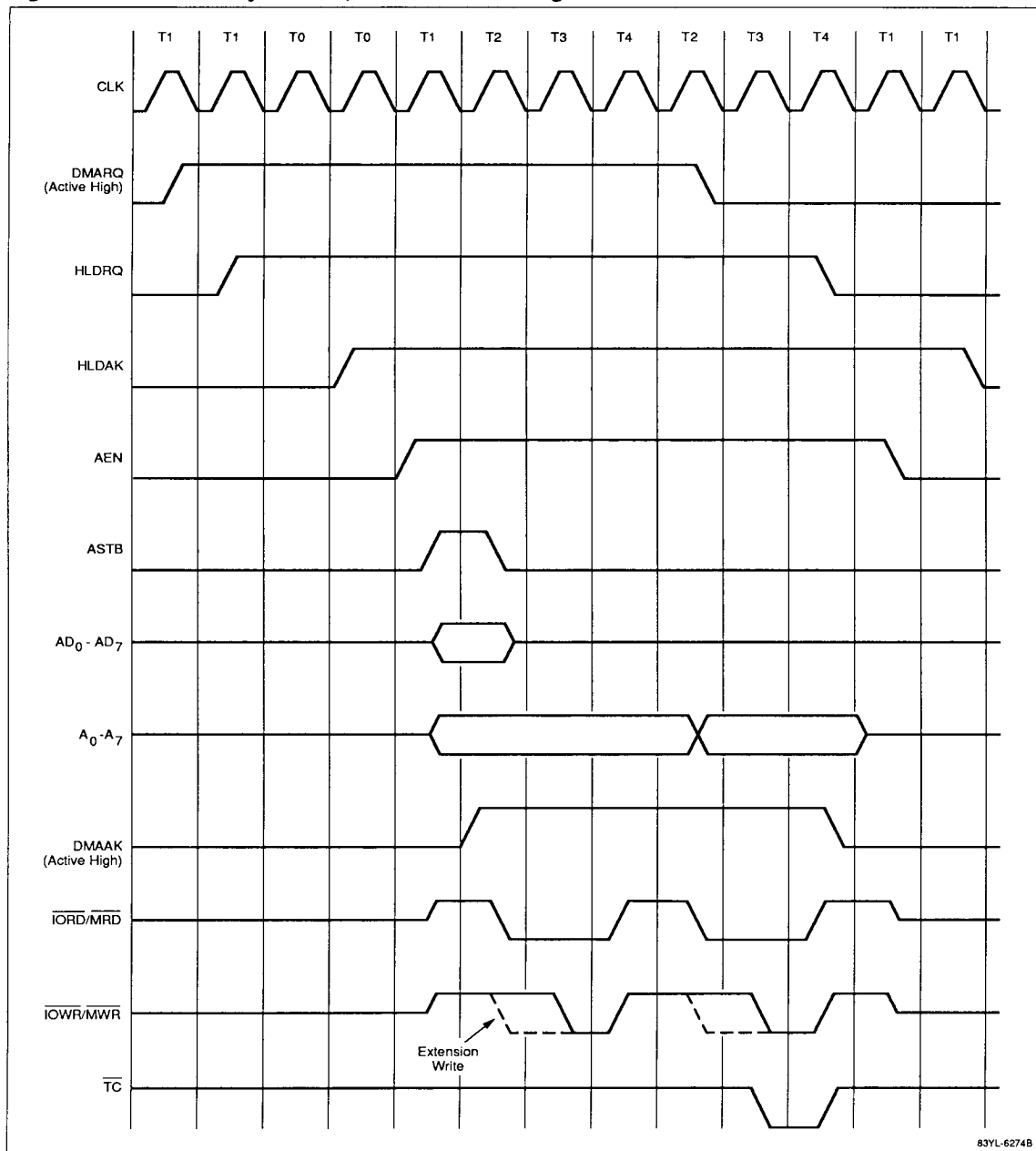
Figure 6. I/O-to-Memory Transfer, Normal Mode Timing
