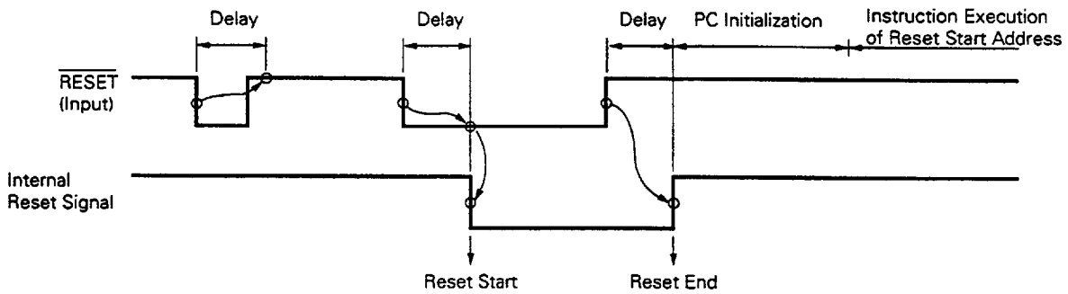
Fig. 3-6 Reset Acknowledge
