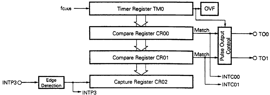
Fig. 2-5 Timer/Counter Unit Block Diagram
