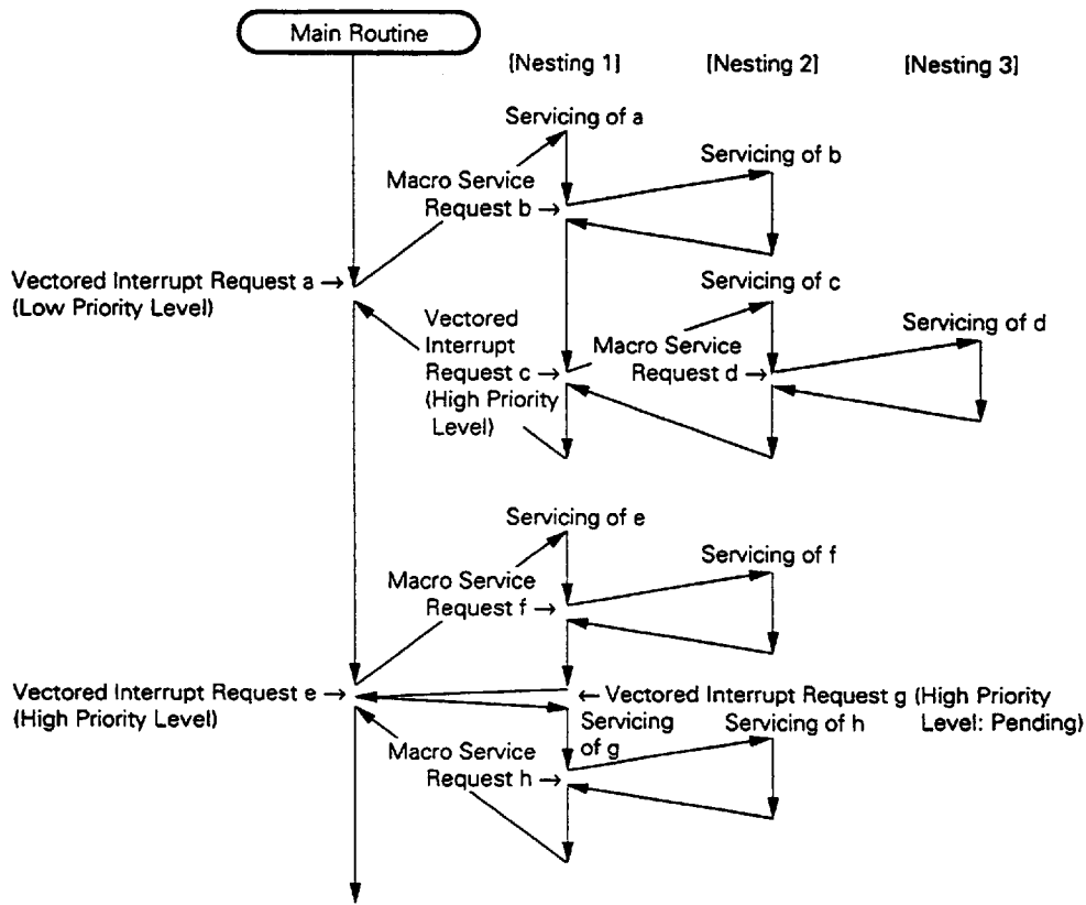
Fig. 3-1 Servicing Example for Another Interrupt Request Occurrence while an Interrupt Servicing
