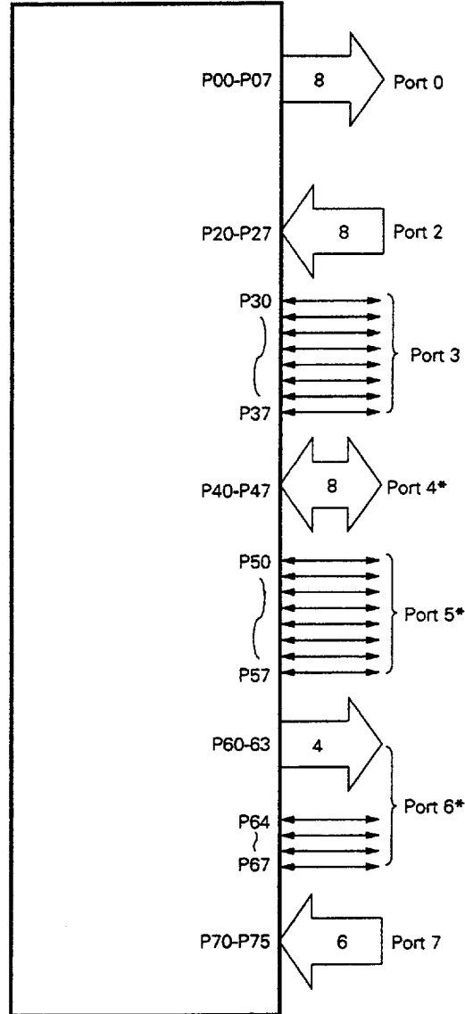
Fig. 2-3 Port Configuration
