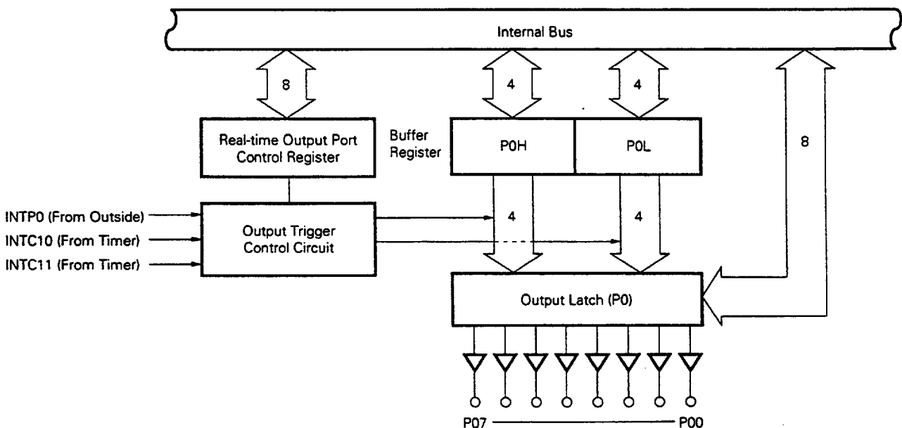
Fig. 2-4 Real-Time Output Port Block Diagram
