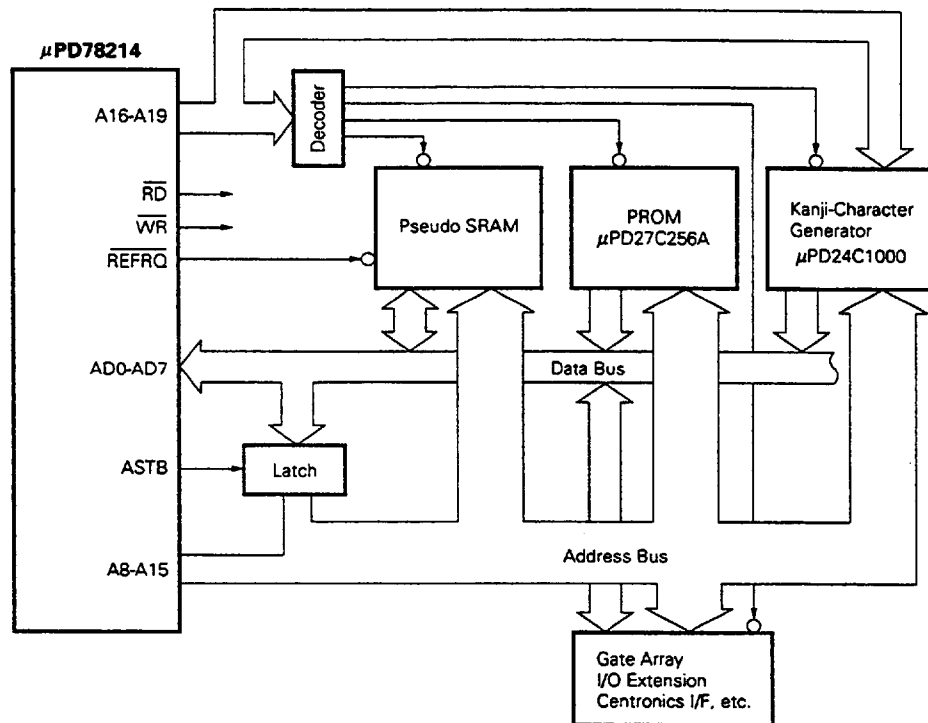
Fig. 3-4 Local Bus Interface Example
