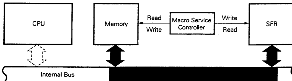
Fig. 3-3 Macro Service
