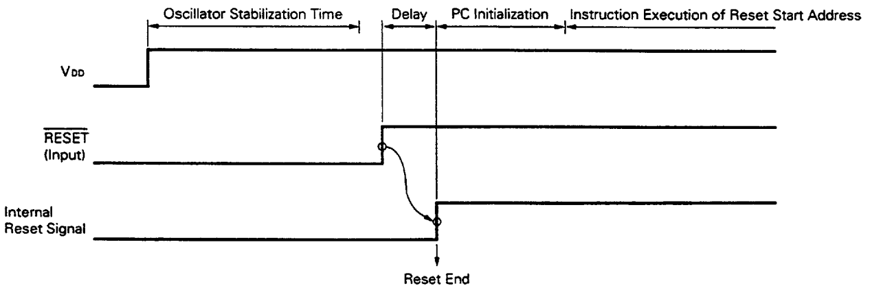
Fig. 3-7 Reset Operation at Power-On
