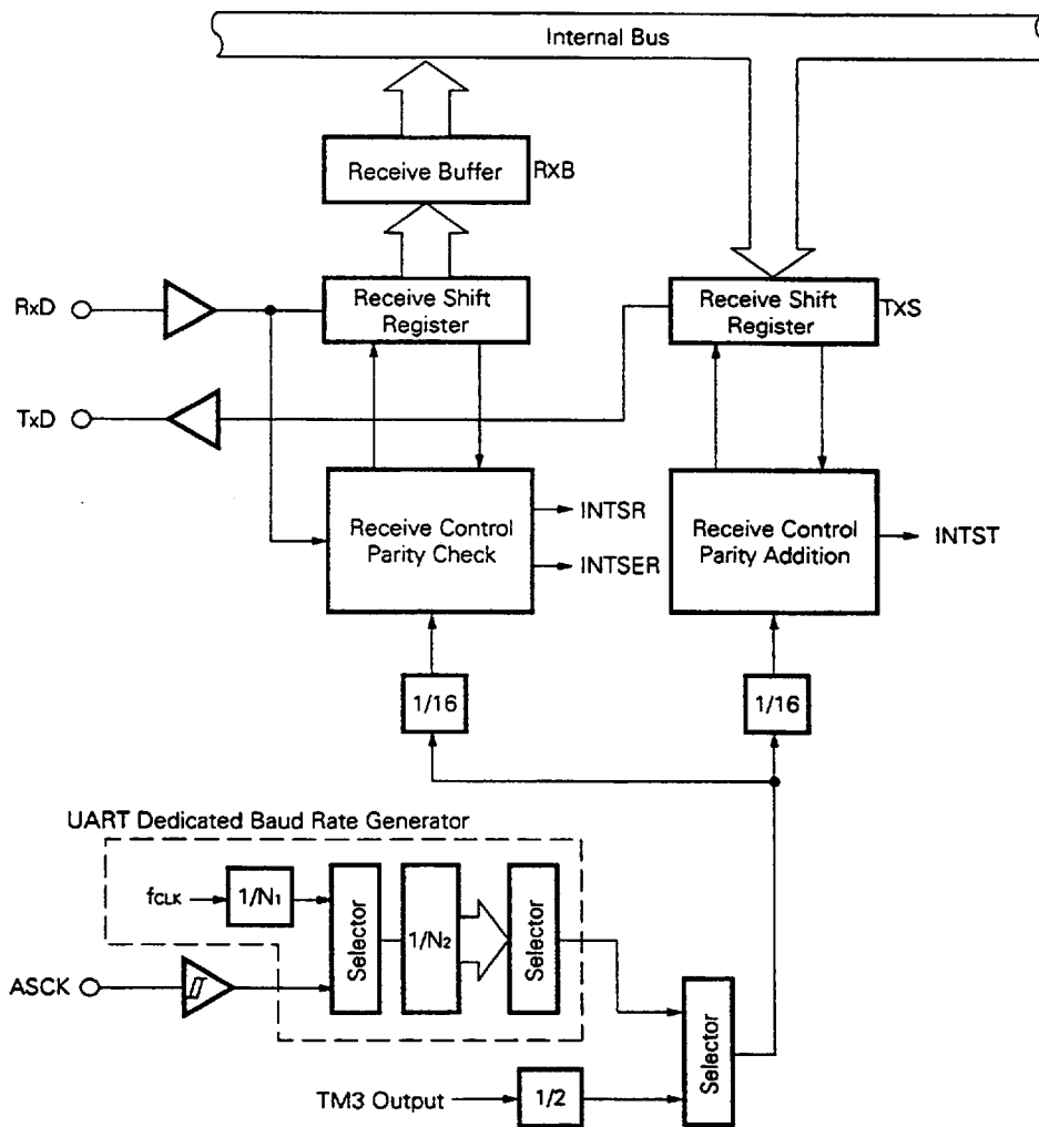
Fig. 2-8 Asynchronous Serial Interface Block Diagram
