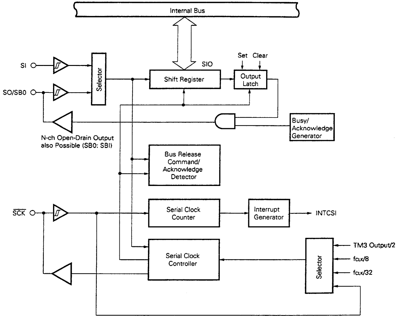
Fig. 2-9 Clocked Serial Interface Block Diagram
