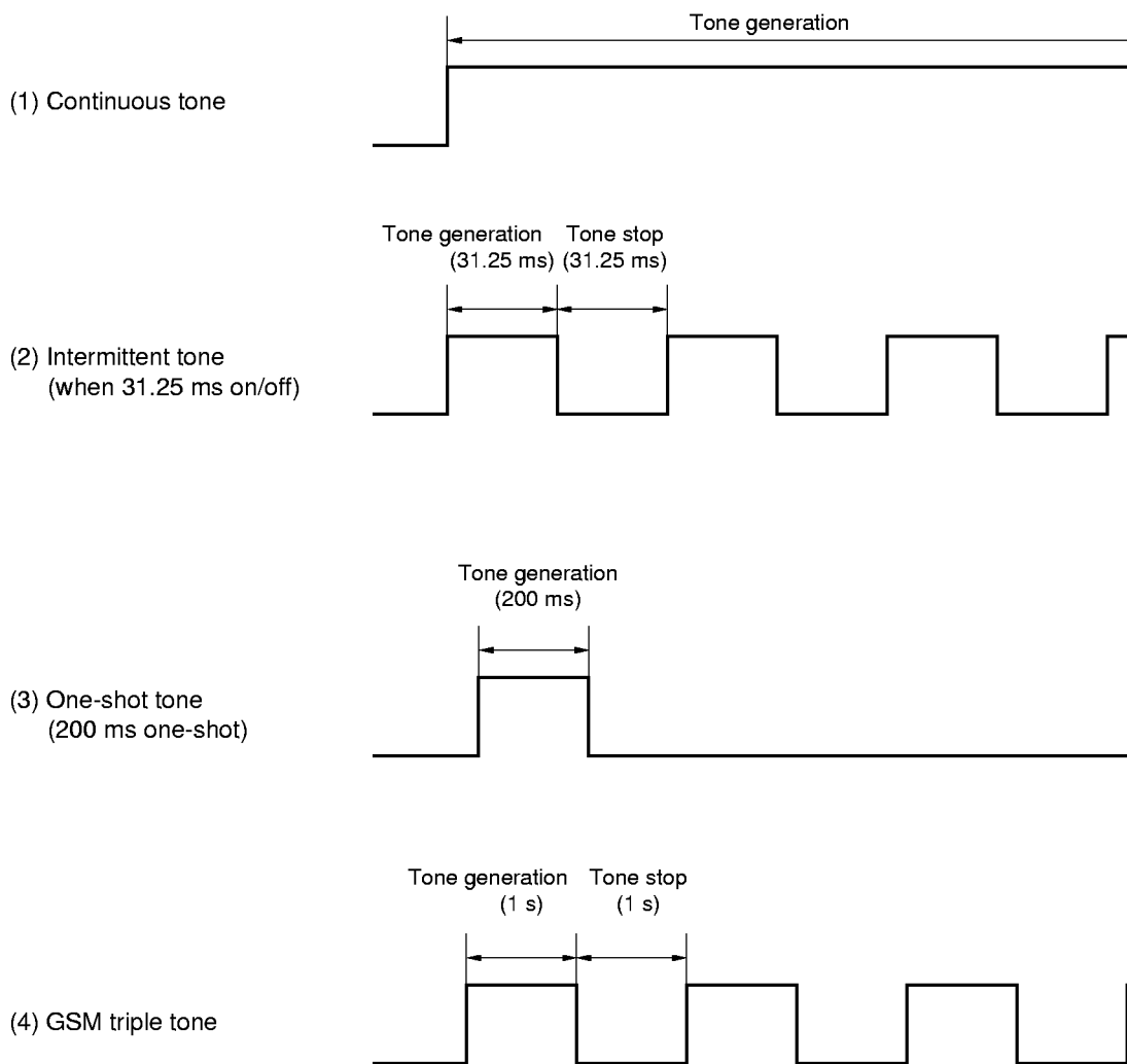
Figure 3-1 Tone Interval Output Waveform
