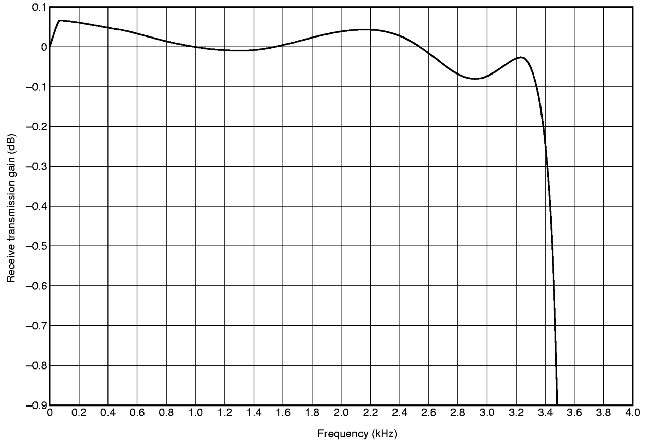
Receive Transmission Gain Frequency Characteristics 2 (GRR)
