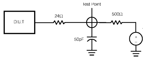
Load for Enable and Disable Times
