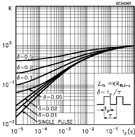
Thermal Impedance For SOT82-FM
