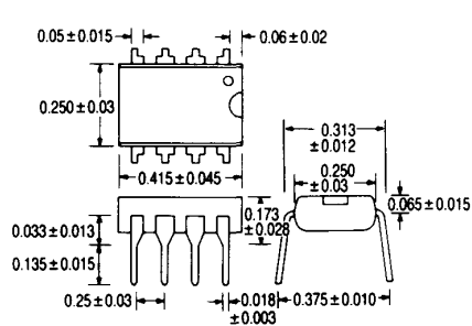
8-pin plastic DIP
