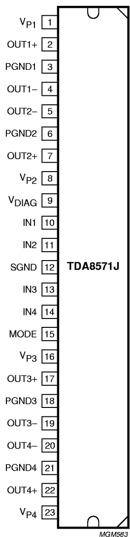
Fig.2 Pin configuration.
