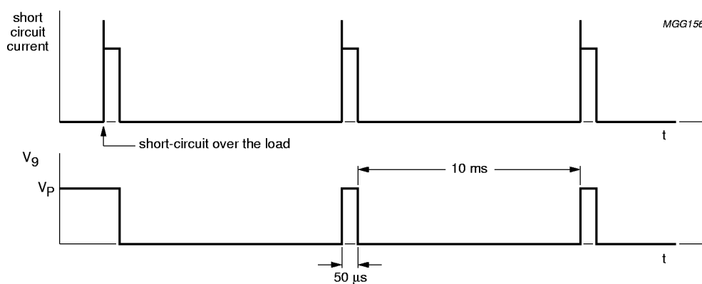
Fig.5 Short-circuit waveform.
