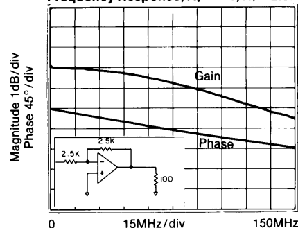
Frequency Response, A_V = -1 , R_i = 2.5k\Omega
