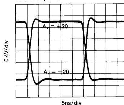
Pulse Response
