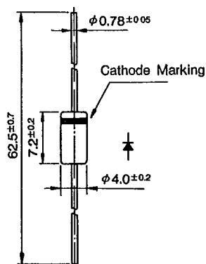
Outline Drawing ③⑨
