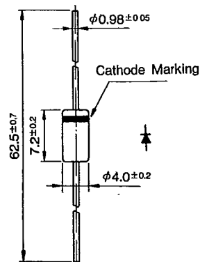
Outline Drawing ④①
