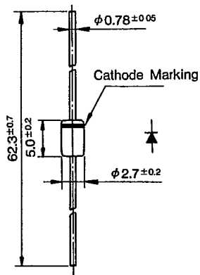
Outline Drawing ③⑨
