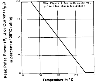
FIGURE 4 DERATING CURVE
