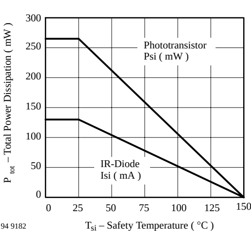
Figure 1. Derating diagram
