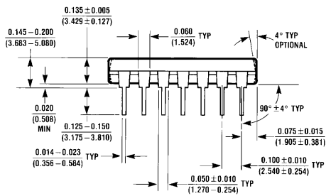
14-Lead Molded Dual-In-Line Package (N) Order Number DM74LS38N NS Package Number N14A
