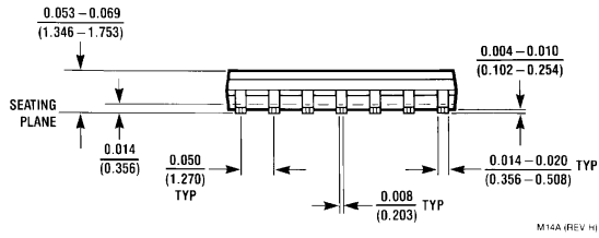
14-Lead Small Outline Molded Package (M) Order Number DM74LS38M NS Package Number M14A
