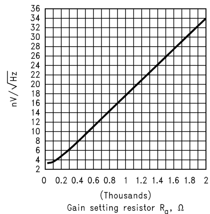
FIGURE 5. Equivalent Input Noise Voltage ( e_n ) vs. R_g
