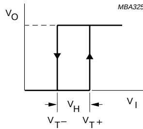
Fig.6 Transfer characteristic.
