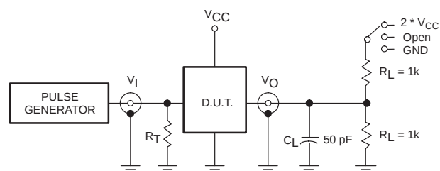
Test Circuit for Outputs
