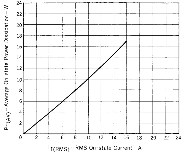
Fig. 10 P_{T(AV)} - I_{T(RMS)} CHARACTERISTIC
