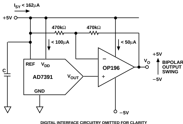
Figure 27. Bipolar Output Operation
