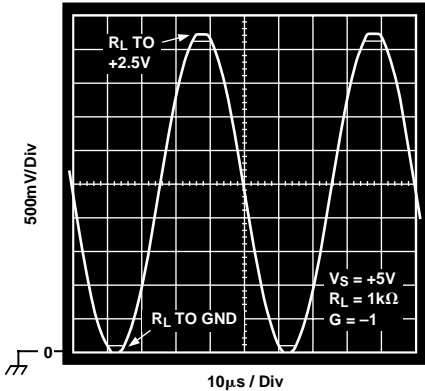
Figure 33. Output Swing
