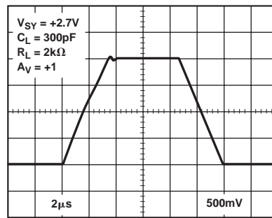
Figure 17. Large Signal Transient Response at +2.7 V
