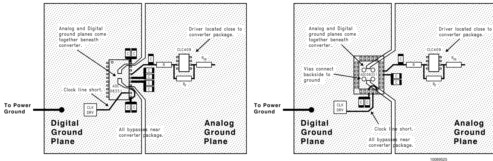
FIGURE 3. Layout examples showing separate analog and digital ground planes connected below the ADC08351.
