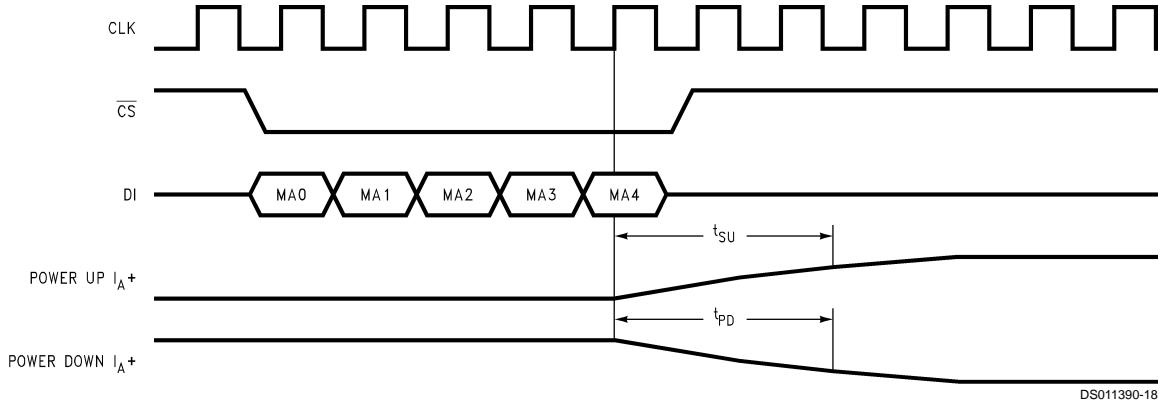
FIGURE 7. Software Power Up/Down Sequence
