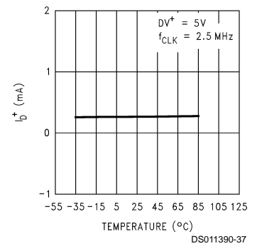
Digital Supply Current ( I_{D+} ) vs Temperature
