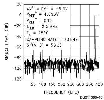
Power Bandwidth Response with 380 kHz Sine Wave
