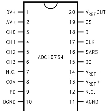
See NS Package Number MSA20
