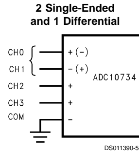
FIGURE 13. Analog Input Multiplexer Options
