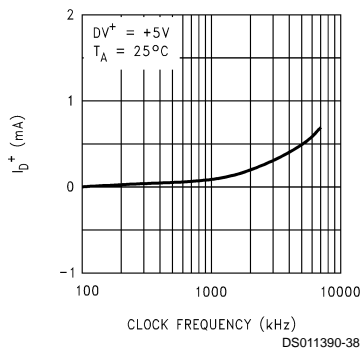
Digital Supply Current ( I_{D+} ) vs Clock Frequency
