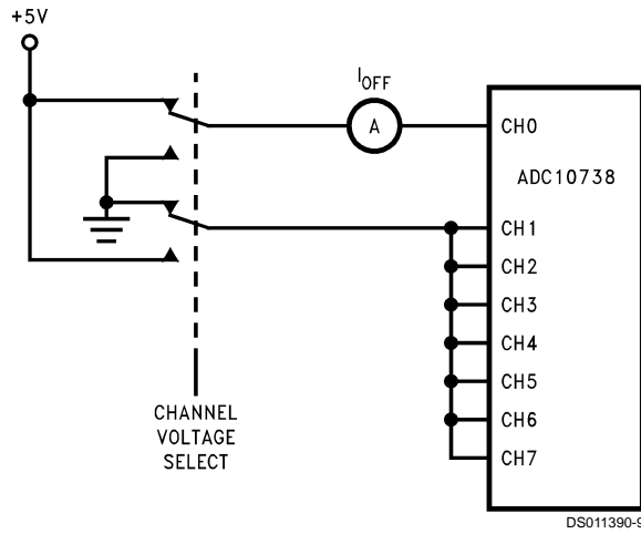
Leakage Current Test Circuit
