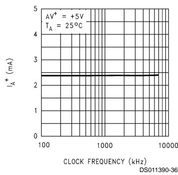
Analog Supply Current ( I_{A+} ) vs Clock Frequency
