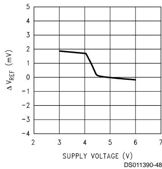
Line Regulation
