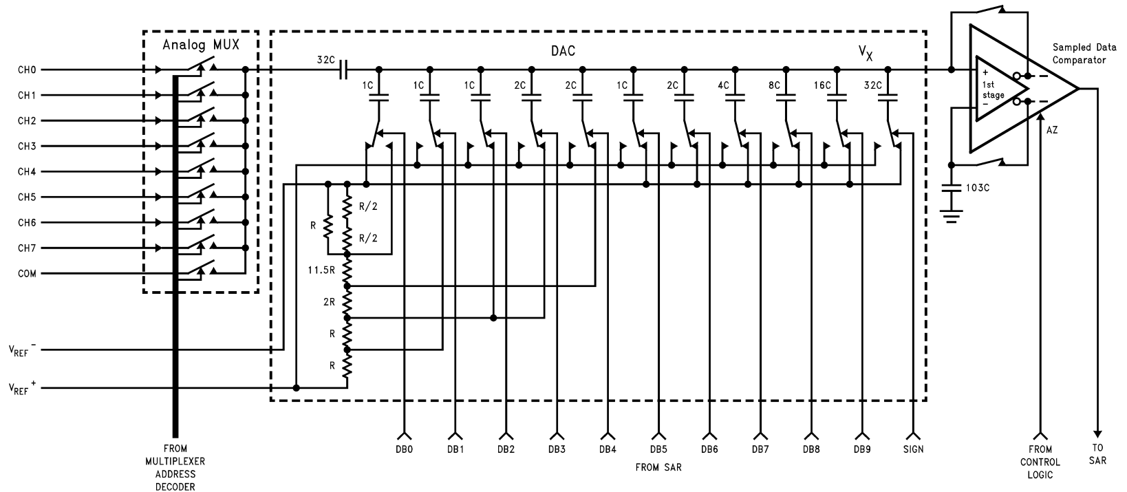
FIGURE 12. Detailed Diagram of the ADC10738 DAC and Analog Multiplexer Stages
