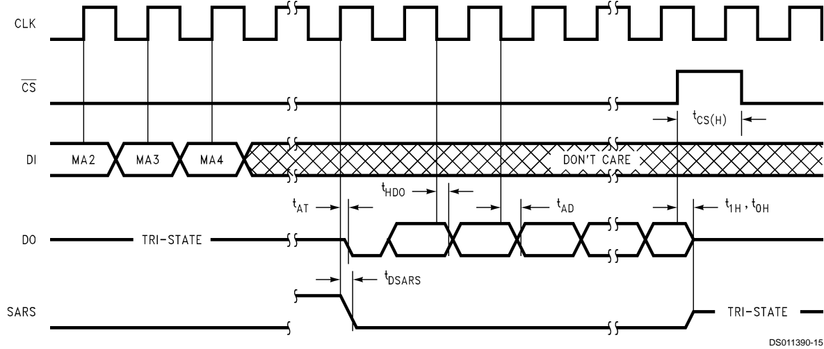
FIGURE 4. DO Timing
