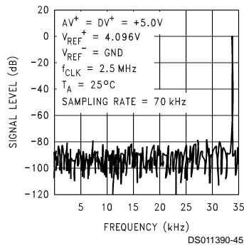
Spectral Response with 34 kHz Sine Wave
