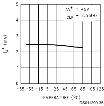
Analog Supply Current ( I_{A+} ) vs Temperature
