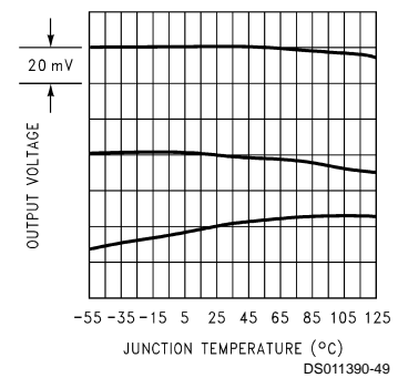
Output Drift vs Temperature (3 Typical Parts)
