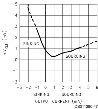
Load Regulation
