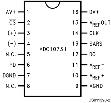
Top View See NS Package Number M16B
