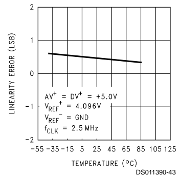
Linearity Error vs Temperature
