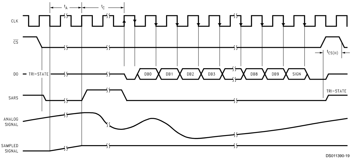
FIGURE 8. ADC10731 CS Low during Conversion
