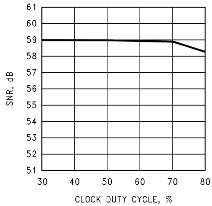
SNR vs. Clock Duty Cycle @ f_{IN} = 4.7 MHz
