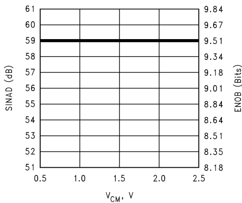
SINAD & ENOB vs. V_{CM} @ f_{IN} = 9.5\text{ MHz}
