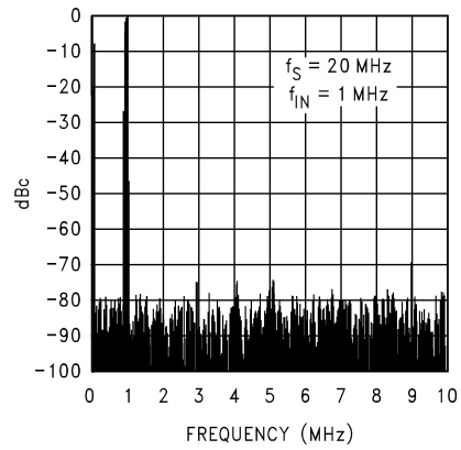
Spectral Response @ f_{IN} = 1\text{ MHz}
