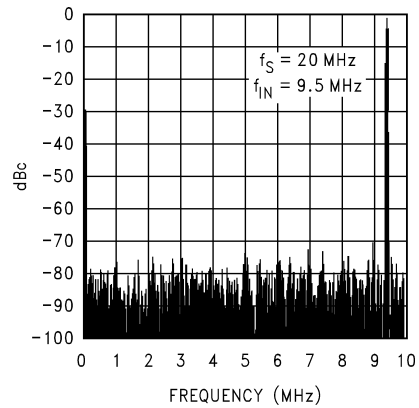
Spectral Response @ f_{IN} = 9.5\text{ MHz}
