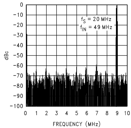
Spectral Response @ f_{IN} = 49\text{ MHz}
