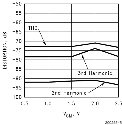
Distortion vs. V_{CM} @ f_{IN} = 4.7 MHz
