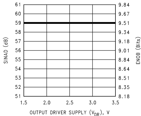
SINAD & ENOB vs. V_{DR} @ f_{IN} = 9.5\text{ MHz}
