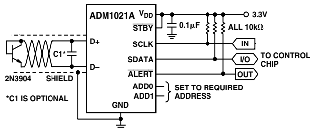
Figure 18. Typical ADM1021A Application Circuit
