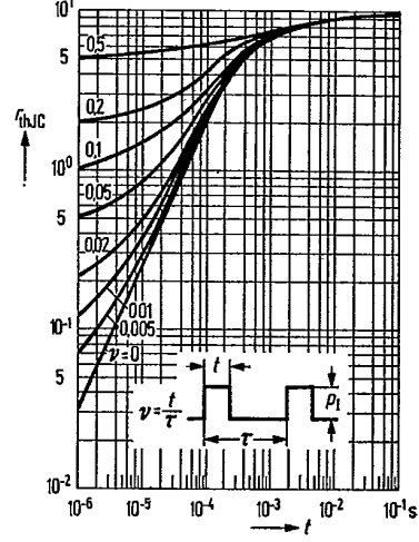
Permissible pulse load r_{thJC} = f(t); v = \text{parameter} BD 135, BD 137, BD 139
