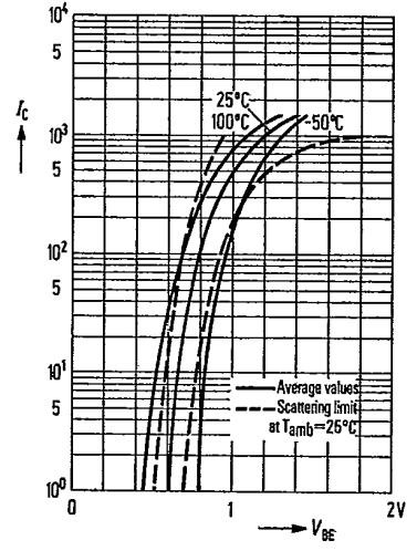
Collector current I_C = f(V_{BE}) V_{CE} = 2\text{V}; T_{amb} = \text{parameter} (common emitter configuration) BD 135, BD 137, BD 139
