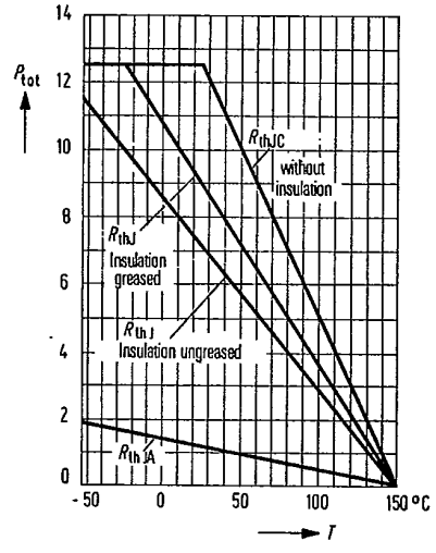
Total perm. power dissipation versus temperature P_{tot} = f(T); R_{th} = \text{parameter} BD 135, BD 137, BD 139
