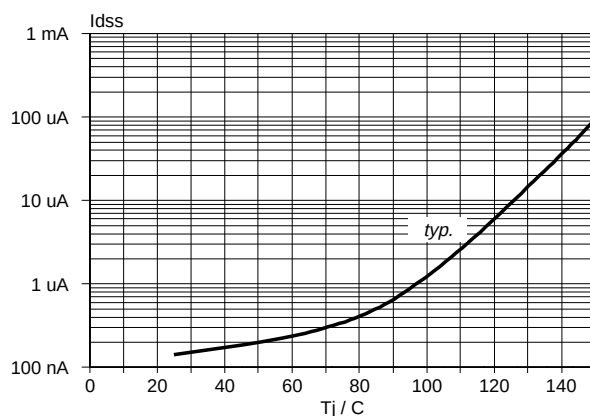
Fig.20. Typical off-state leakage current. I_{DSS} = f(T_j) ; Conditions: V_{DS} = 40\text{ V} ; I_{IS} = 0\text{ V} .
