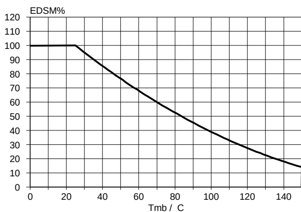
Fig.18. Normalised limiting clamping energy. E_{DSM}\% = f(T_{mb}) ; conditions: I_D = 15\text{ A} ; V_{IS} = 5\text{ V}
