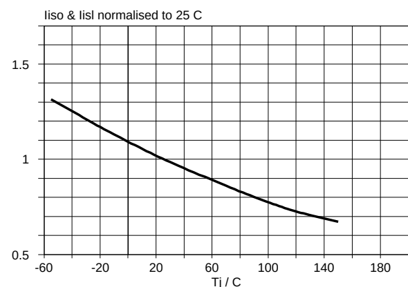
Fig.21. Normalised input currents (normal & latched). I_{ISO}/I_{ISO\ 25^\circ\text{C}} \text{ \& } I_{ISL}/I_{ISL\ 25^\circ\text{C}} = f(T_j) ; V_{IS} = 5\text{ V}
