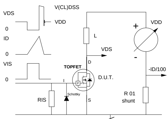
Fig.19. Clamping energy test circuit, R_{IS} = 50\ \Omega . E_{DSM} = 0.5 \cdot L I_D^2 \cdot V_{(CL)DSS} / (V_{(CL)DSS} - V_{DD})
