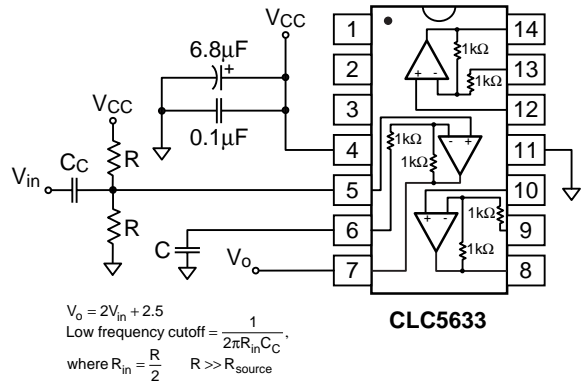
Figure 5: AC Coupled, A_v = +1/V Configuration
