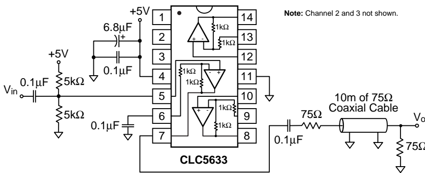
Figure 13: Single Supply Cable Driver
