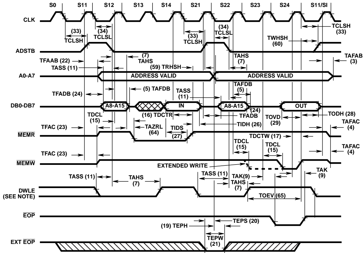
FIGURE 13. MEMORY-TO-MEMORY TRANSFER
