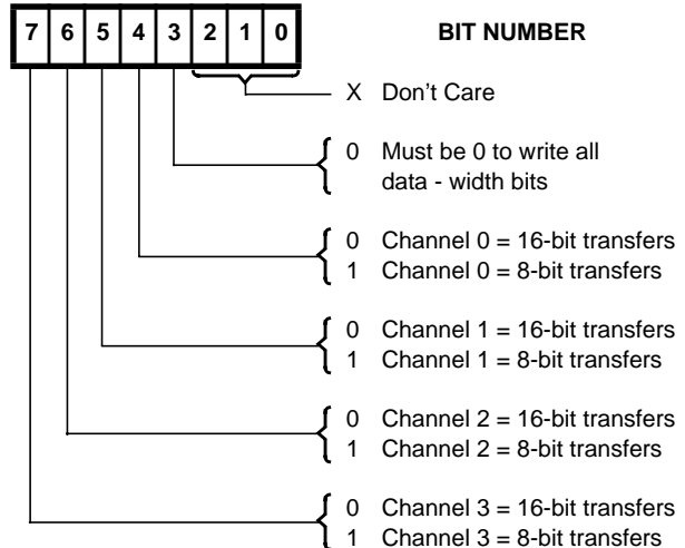
Data-Width Register - 16-bit transfer mode enabled
