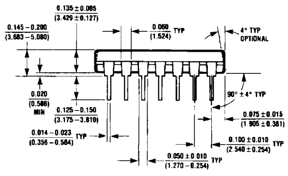
Molded Dual-In-Line Package (N) Order Number DM74ALS132N NS Package Number N14A
