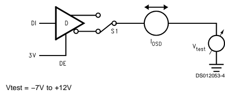
FIGURE 4. Driver I_{OSD}
