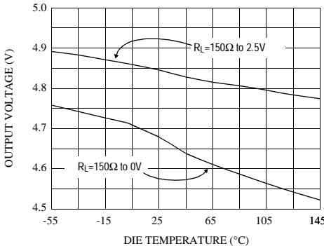
Positive Output Voltage Swing vs. Die Temperature R_L = 150\Omega
