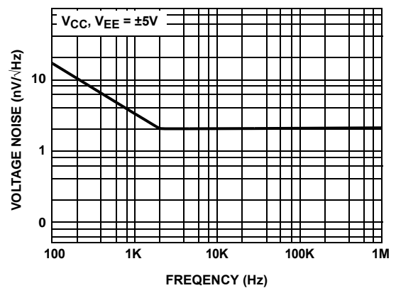
FIGURE 12. VOLTAGE NOISE
