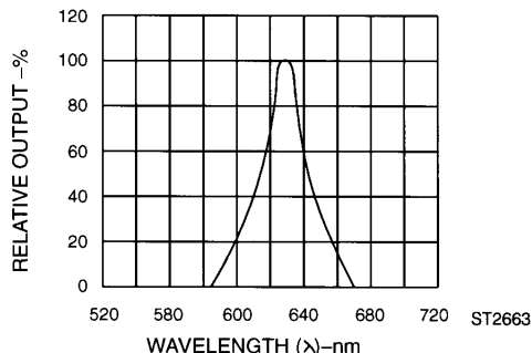
Fig. 2. Spectral Response
