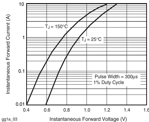
gg1a_03 Figure 3. Typical Instantaneous Forward Characteristics
