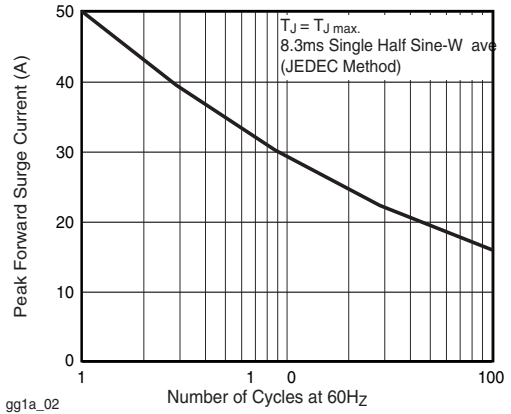
gg1a_02 Figure 2. Maximum Non-Repetitive Peak Forward Surge Current
