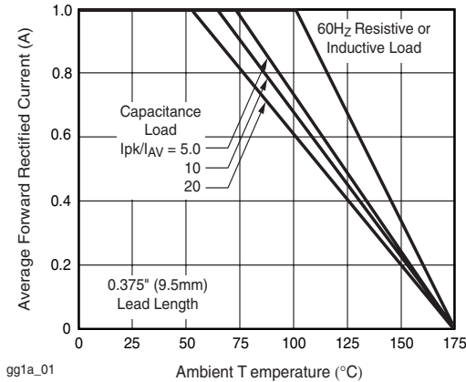
gg1a_01 Figure 1. Forward Current Derating Curve
