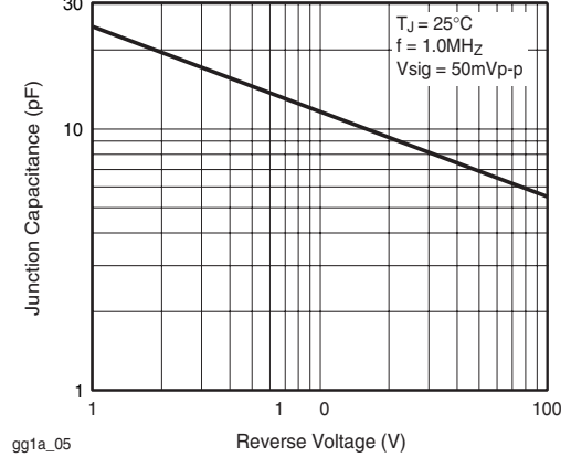
gg1a_05 Figure 5. Typical Junction Capacitance
