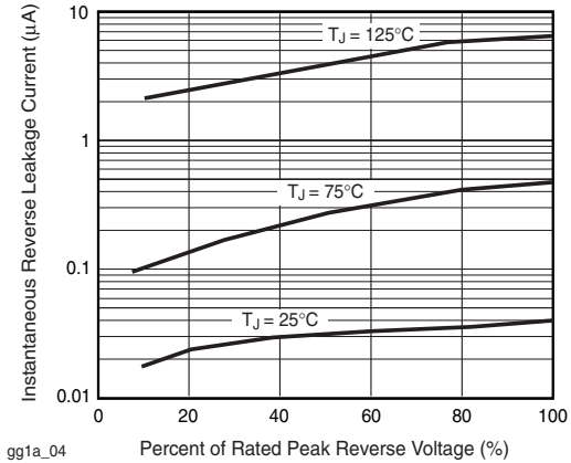
gg1a_04 Figure 4. Typical Reverse Characteristics
