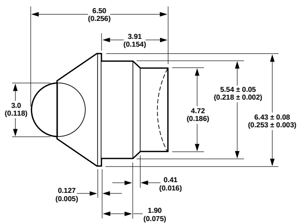
HBCS-A995 Optical Nest Assembly
