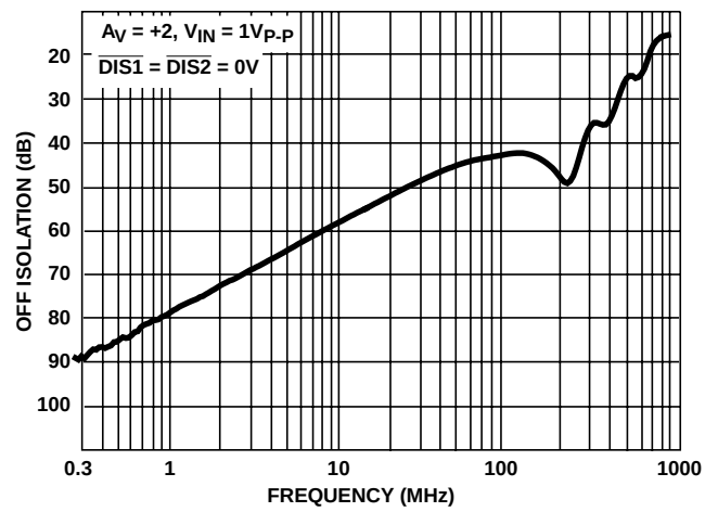
FIGURE 31. ALL HOSTILE OFF ISOLATION
