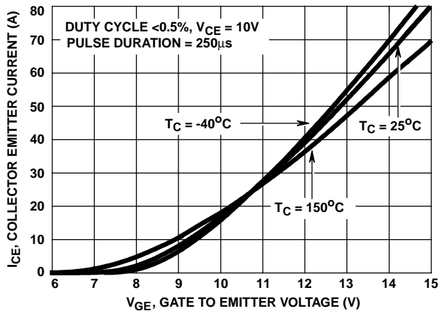
FIGURE 1. TRANSFER CHARACTERISTICS
